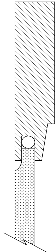
Cross-Section Profile
