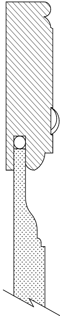
Cross-Section Profile
